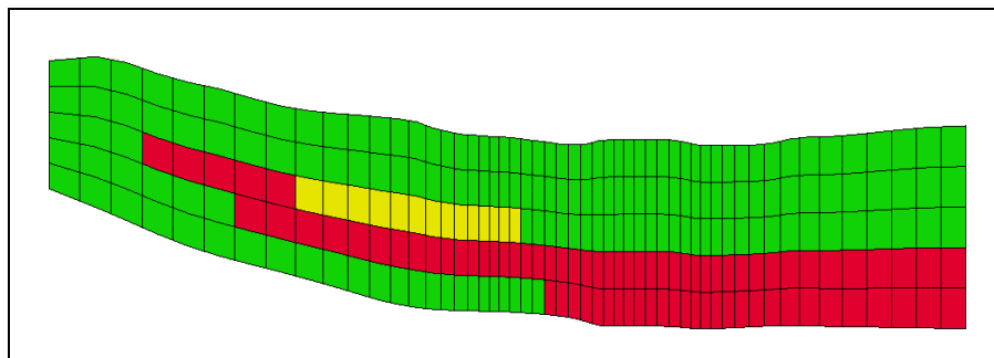
Figure 5. Grid Row after Solids->MODFLOW Using Grid Overlay
