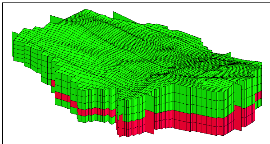
Figure 4. Grid and Solid Cross-sections After Solids→MODFLOW Using Grid Overlay.
