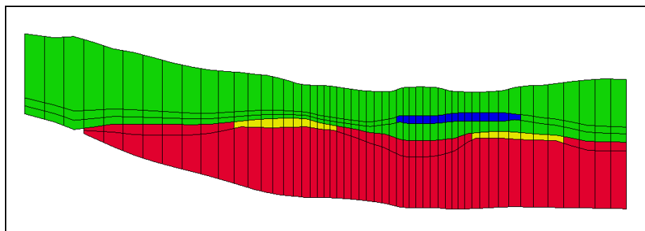
Figure 10. Row 30 of Model Grid Using Target Minimum Thickness and Top Cell Bias
