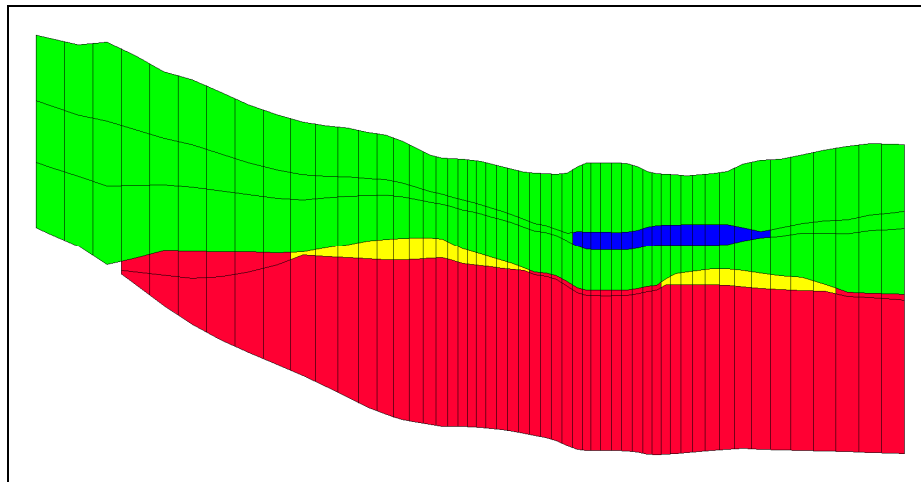
Figure 2. Finite Difference Grid with Elevations and Materials Inherited from Solid Model
